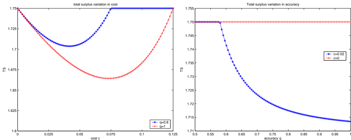
Figure 4: Cost and Accuracy's Impacts on Total Surplus Primitive: V_h = 2 , V_l = 1 , p_l = p_h = \frac{1}{2} .
